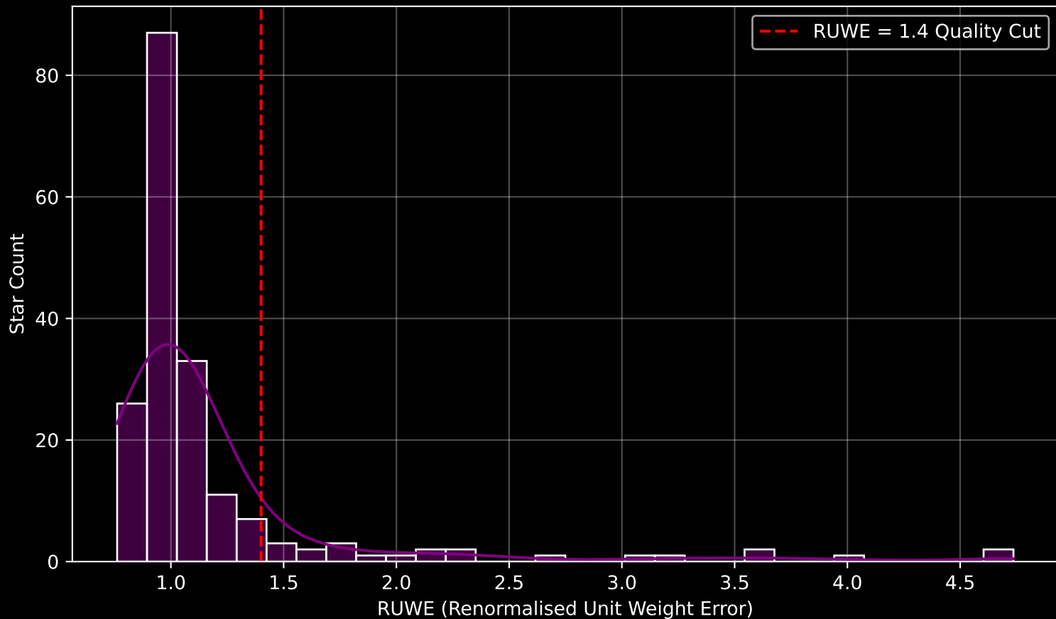
GAPOGEE DR17 Field [122+64_MGA] RUWE Distribution (n= 186)
