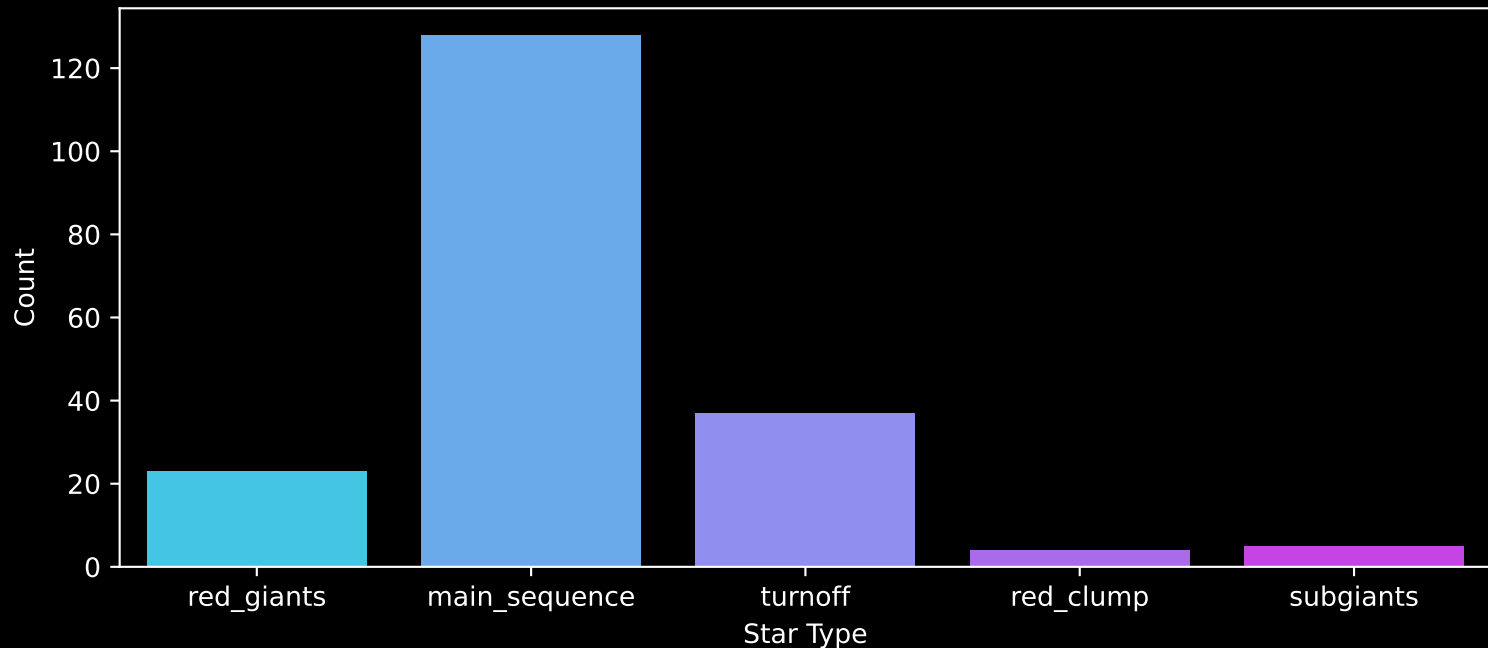
APOGEE DR17 Field: [122+64_MGA] Count plot of Star Type
