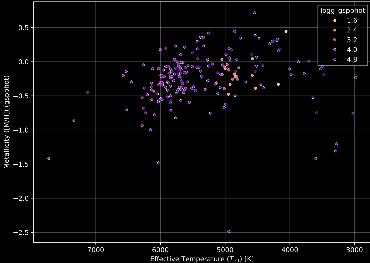
APOGEE DR17 Field: [122+64_MGA] Stellar Population Parameters (n= 197)
