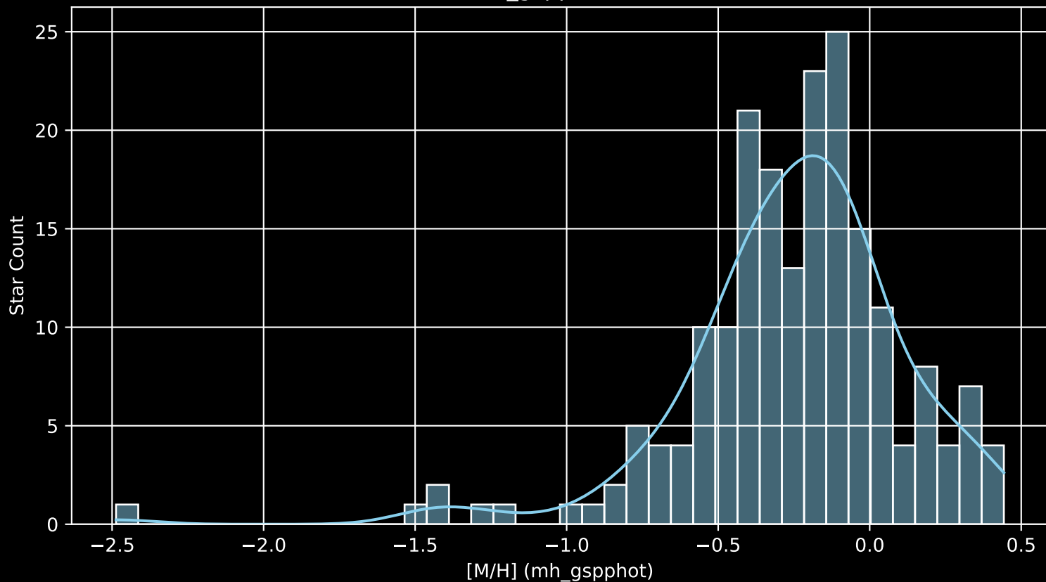
APOGEE DR17 Field: [122+64_MGA [M/H] (mh_gspphot) (n= 196)
