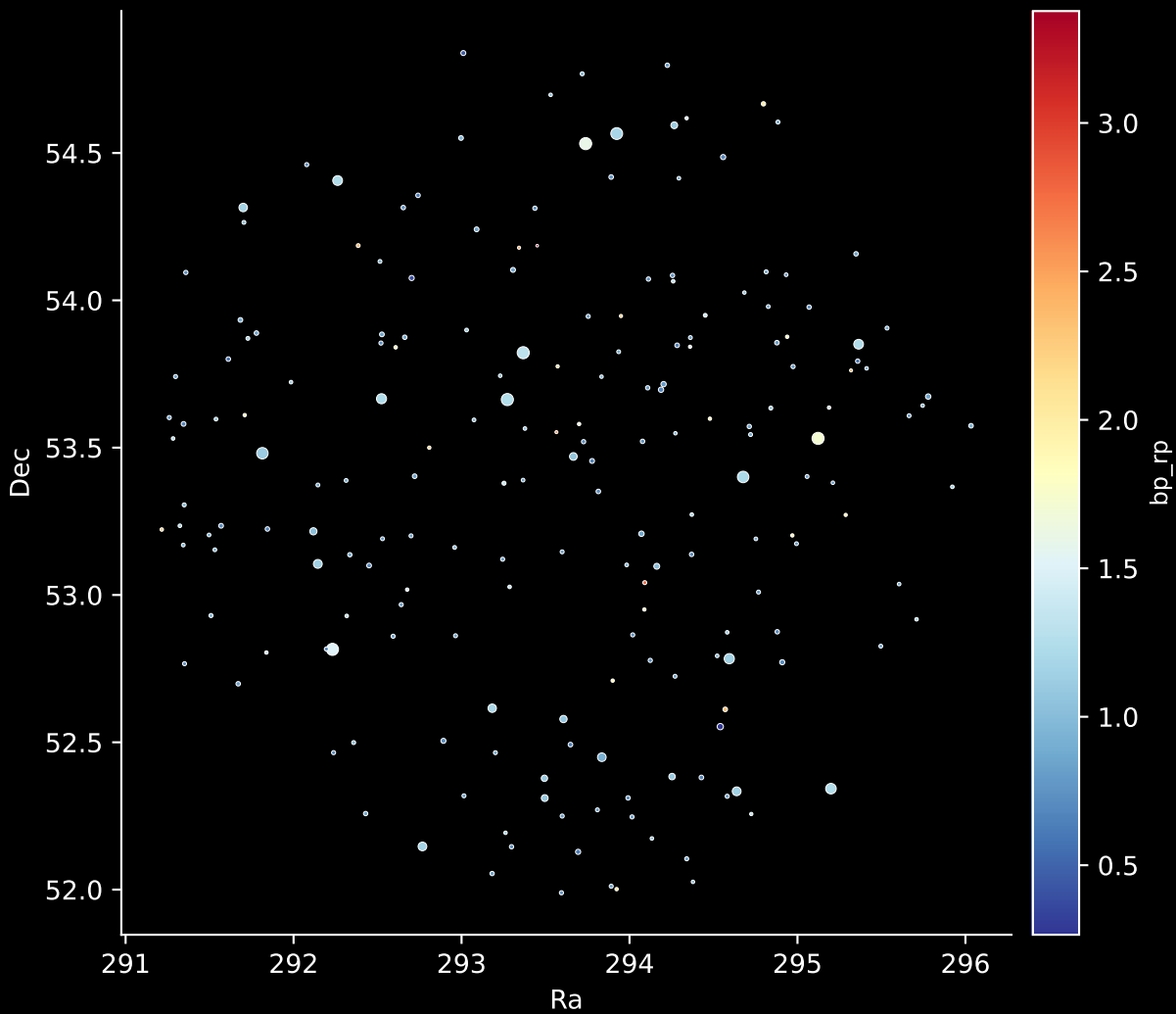
APOGEE DR17 Field: [122+64_MGA] Stars: 197
