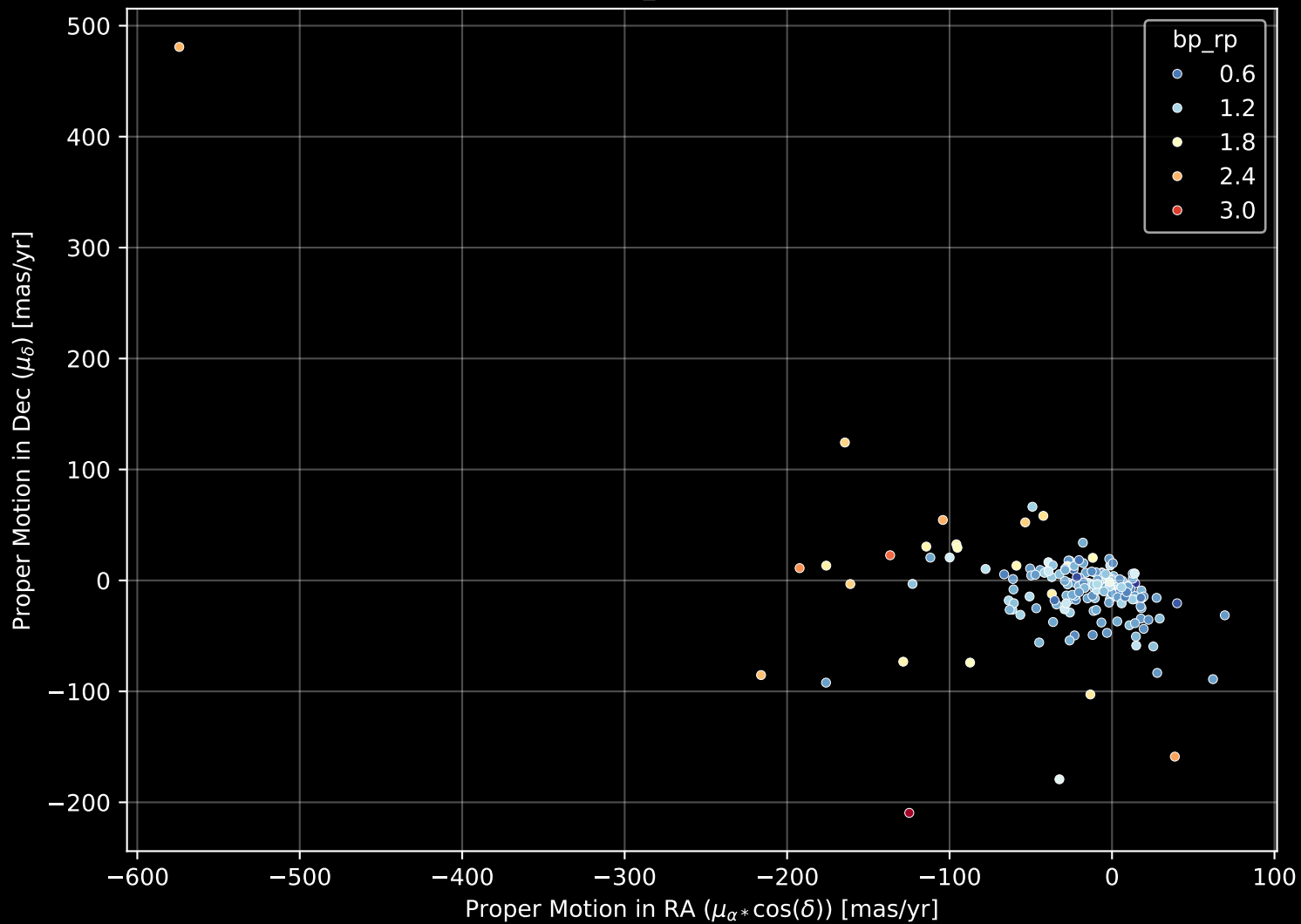
APOGEE DR17 Field: [122+64_MGA] Proper Motion Diagram (n= 197)
