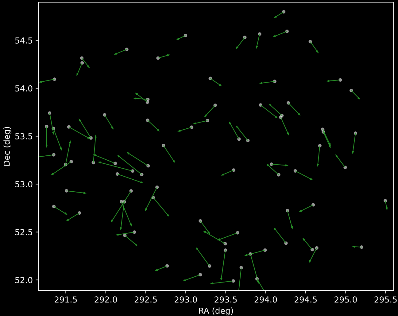
APOGEE DR17 Cluster 4 Proper Motion Vectors (n=81)
