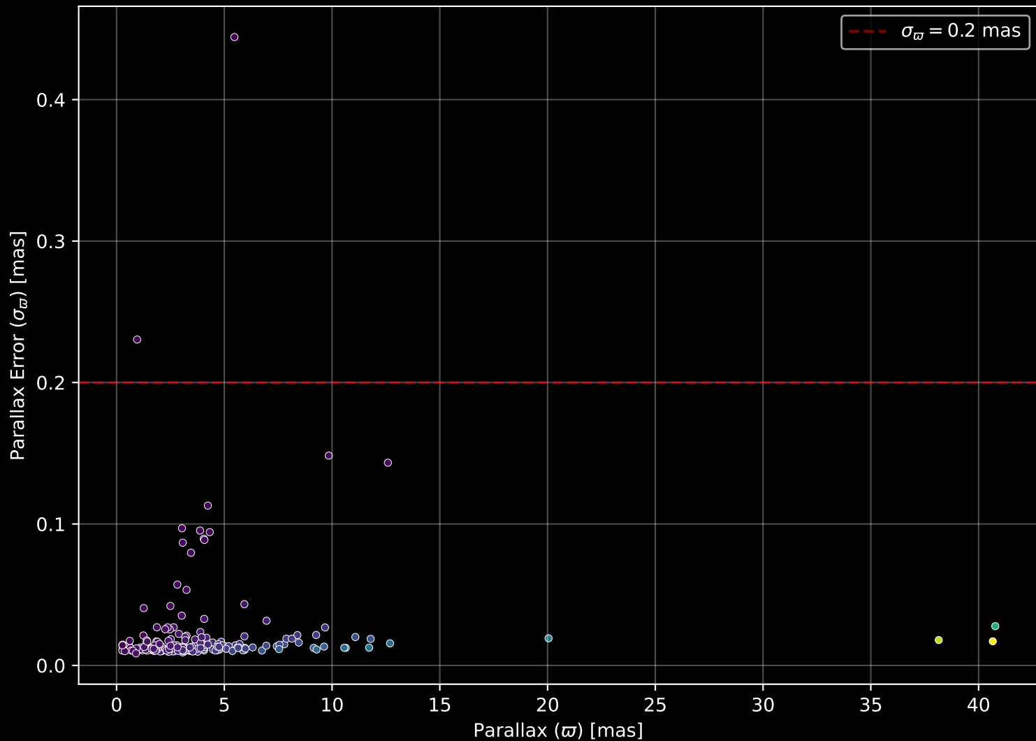
APOGEE DR17 Field: [122+64_MGA] Parallax Quality (n= 197)
